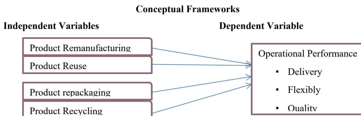
Figure 2.1: Conceptual Frameworks
